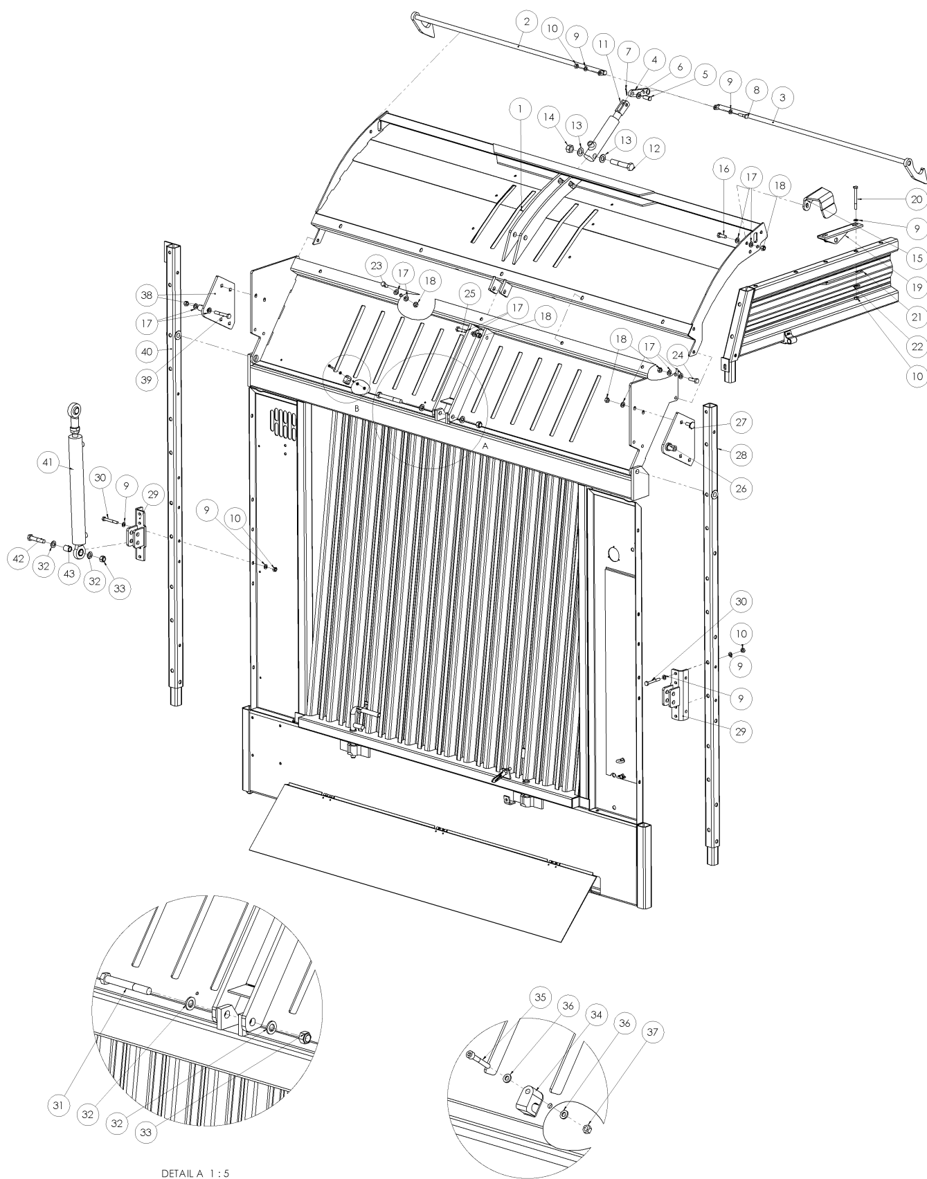
DETAIL A 1:5
